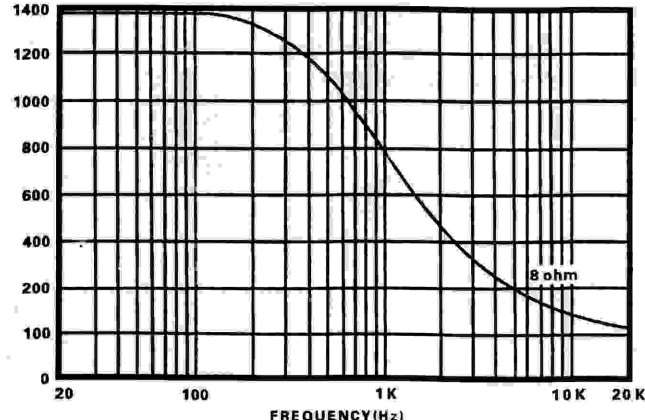
Fig. 6.8 Typical Damping Factor
